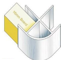
External Corner – GA PLT 1602
