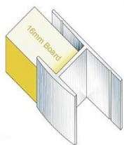
Butt joint – GA PLT 1601
