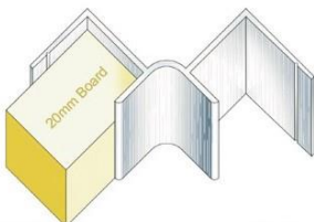
Internal Corner – GA PLT2004
