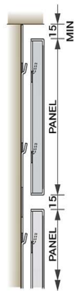
Vertical Section
