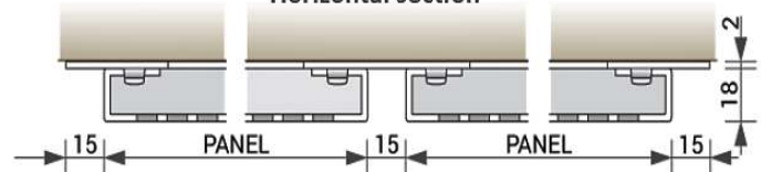
Horizontal section
