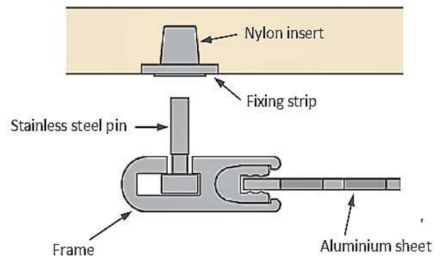
Horizontal section
