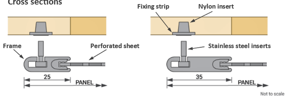
Cross sections
